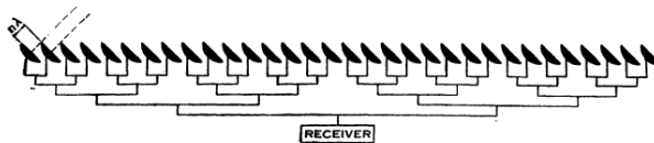
Figure 4: Schematic diagram of the branching transmission lines used for the 32-element solar grating array (after Christiansen and Warburton, 1953a: 192).
