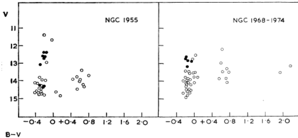
Figure 15: Colour-magnitude diagrams for NGC 1955 and NGC 1968-1974. Open circles represent photographic photometry and the filled circles the Mount Bingar photoelectric magnitudes (after Bok et al., 1962: 492).
