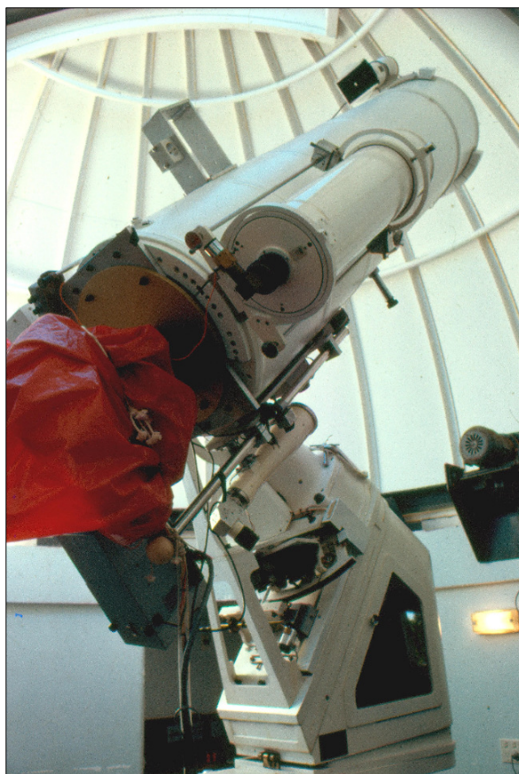
Figure 29: A later view of the Catts Telescope at Perth Observatory, complete with photoelectric photometer and a large new guide scope (courtesy: Graeme White).
