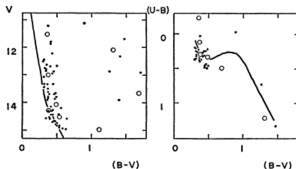
Figure 19: Colour-magnitude and two-colour diagrams for stars in Melotte 105 (after Sher, 1965: 256).
