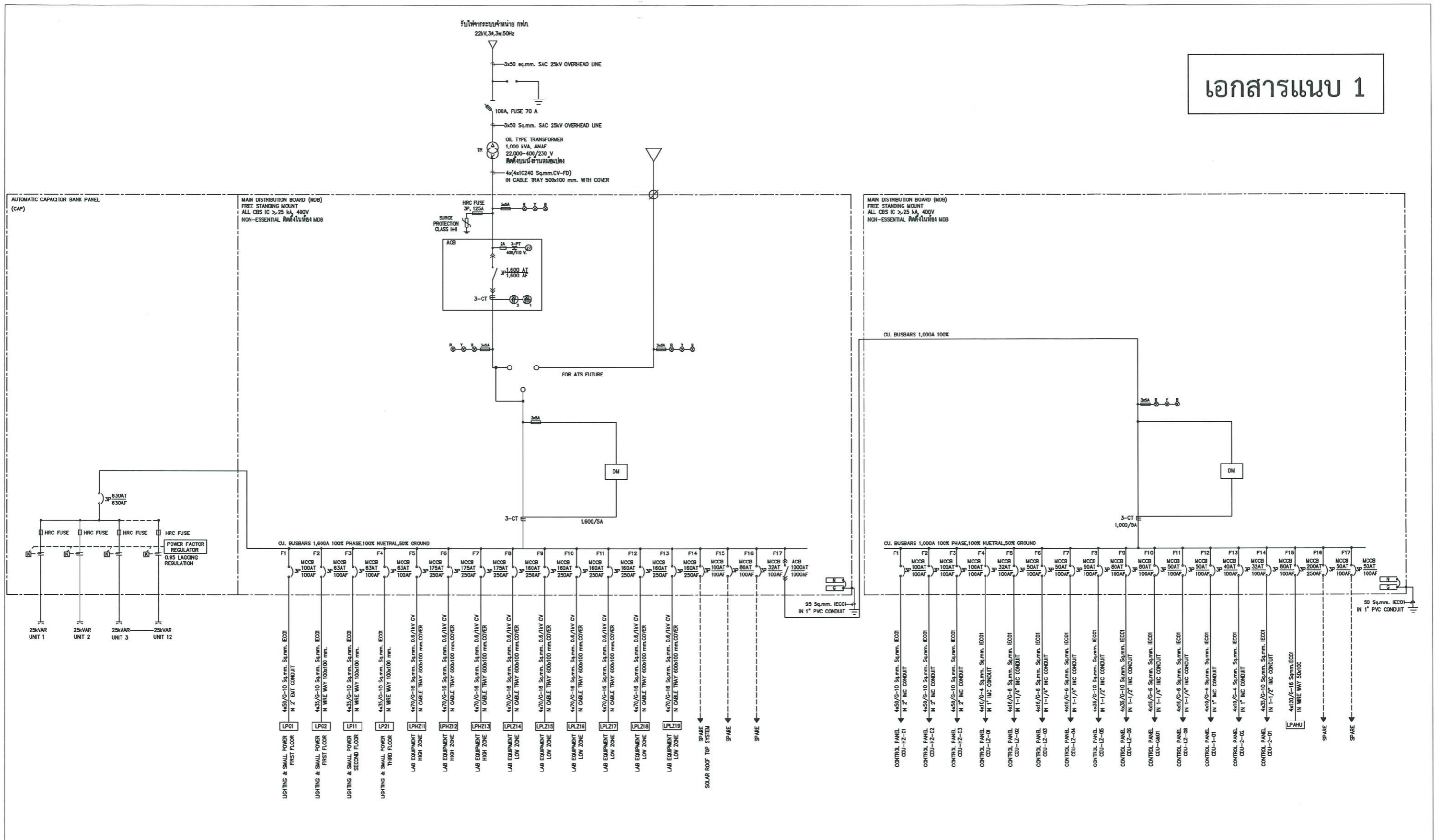
LV SINGLE LINE DIAGRAM SCALE NTS
